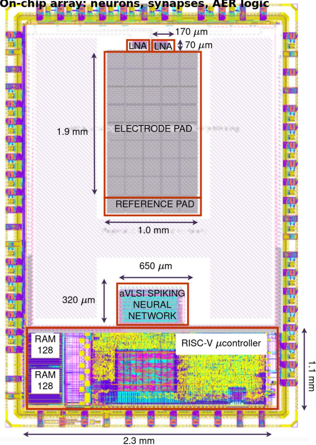
On-chip array: neurons, synapses, AER logic
