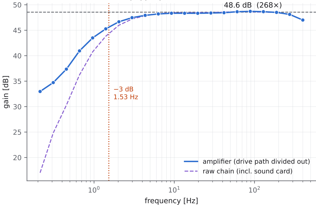
LNA transfer function, 498 \mu\text{Vpp} input
