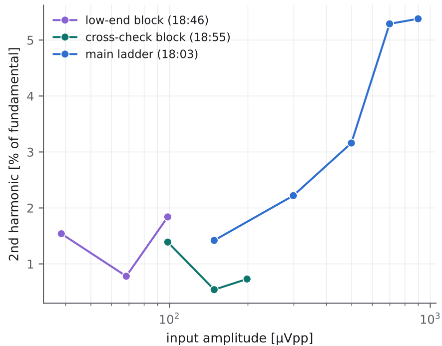
distortion vs input amplitude
