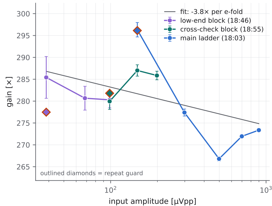
gain vs input amplitude
