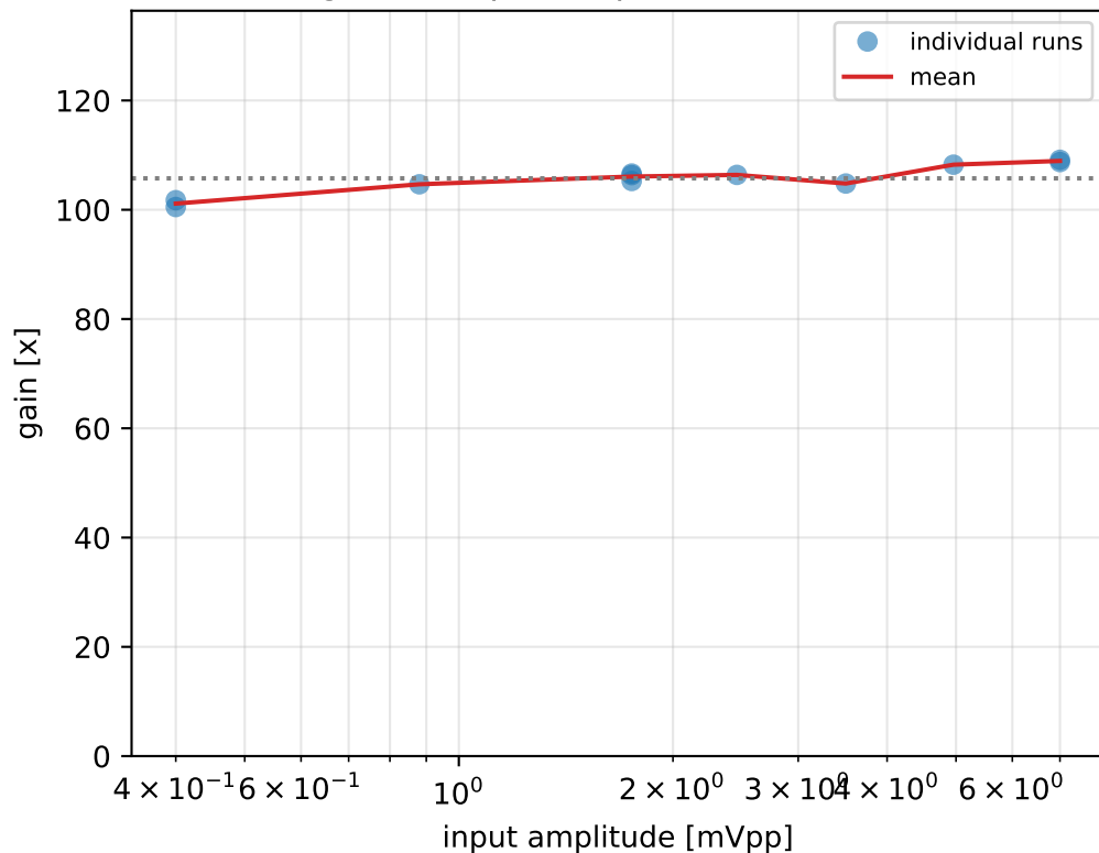
gain vs input amplitude, 88.57 Hz
