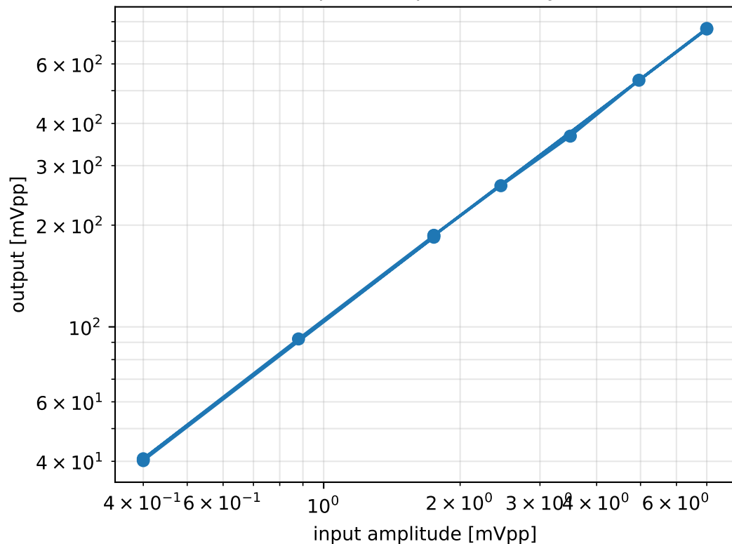
output vs input (linearity)
