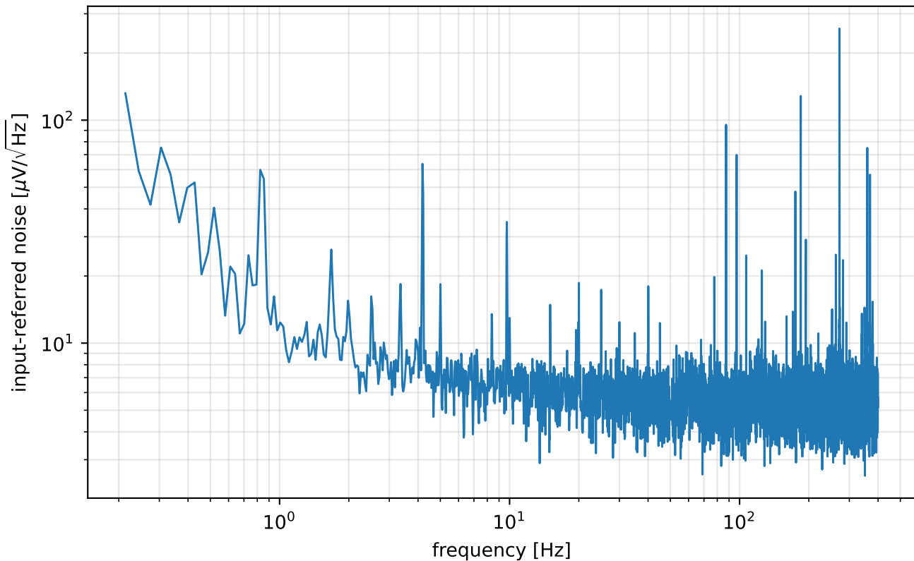
Measured input-referred noise
