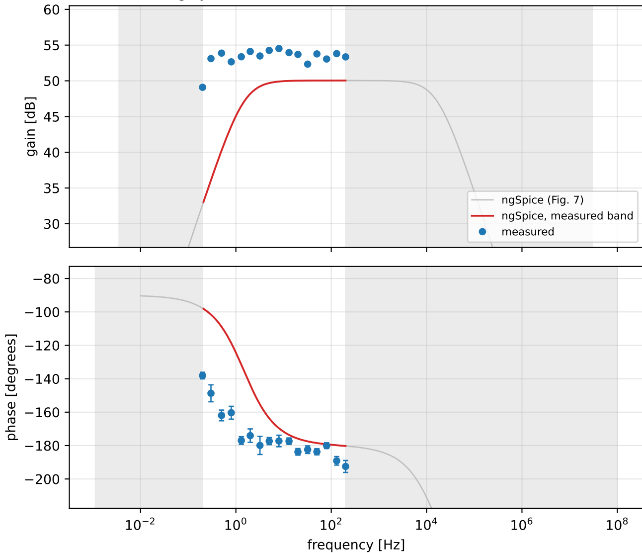
LNA transfer: silicon vs. simulation (grey band = outside what the 1 kS/s bench can reach)
