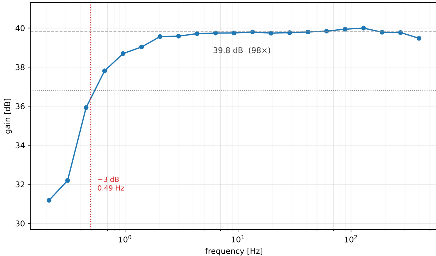
LNA measured transfer function
