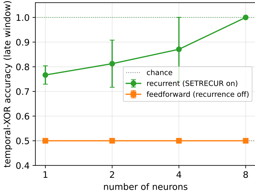
(b) Recurrence \rightarrow memory \rightarrow accuracy
