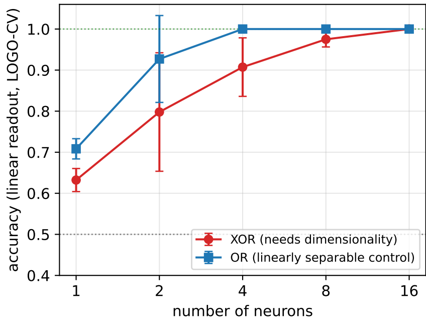
(a) Dimensionality \rightarrow accuracy (XOR)
