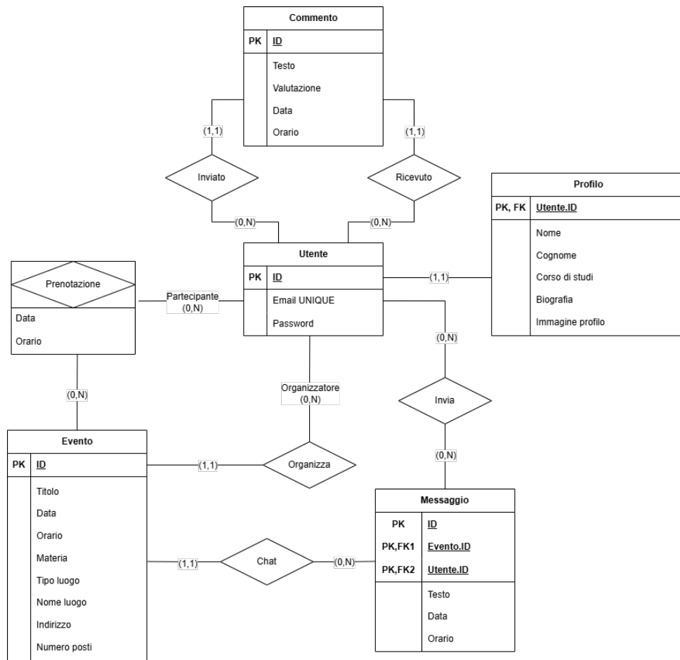
Figura 3.21: Diagramma Entity-Relationship
