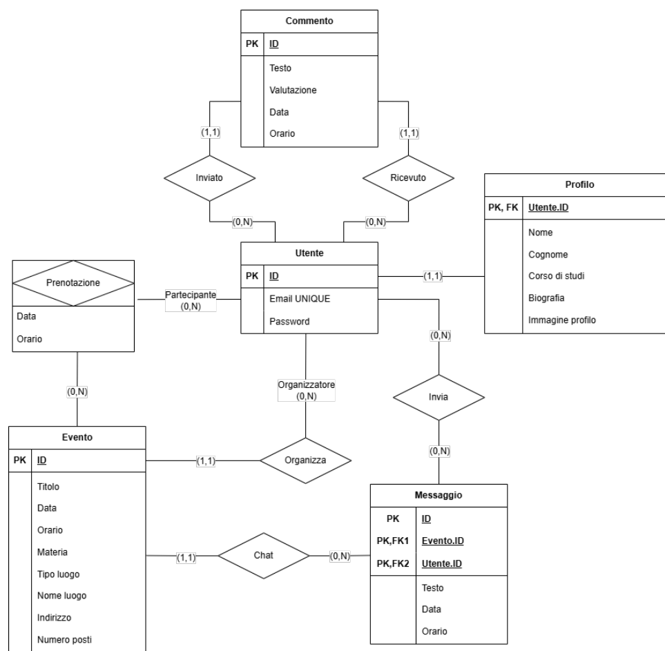
Figura 3.36: Diagramma Entity-Relationship
