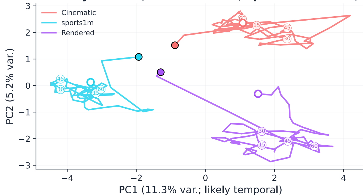
LM: trajectories (filled = frame 0, open = last frame)
