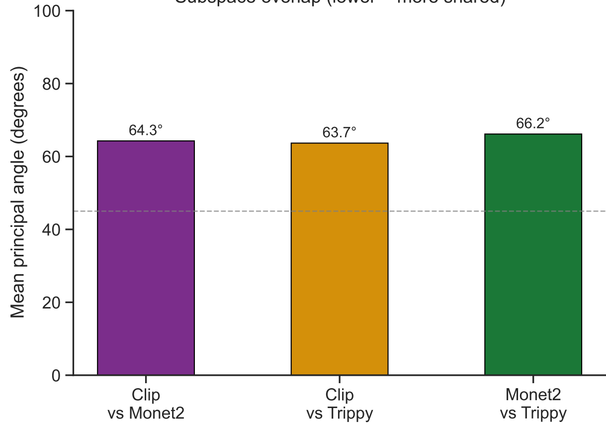
Subspace overlap (lower = more shared)
