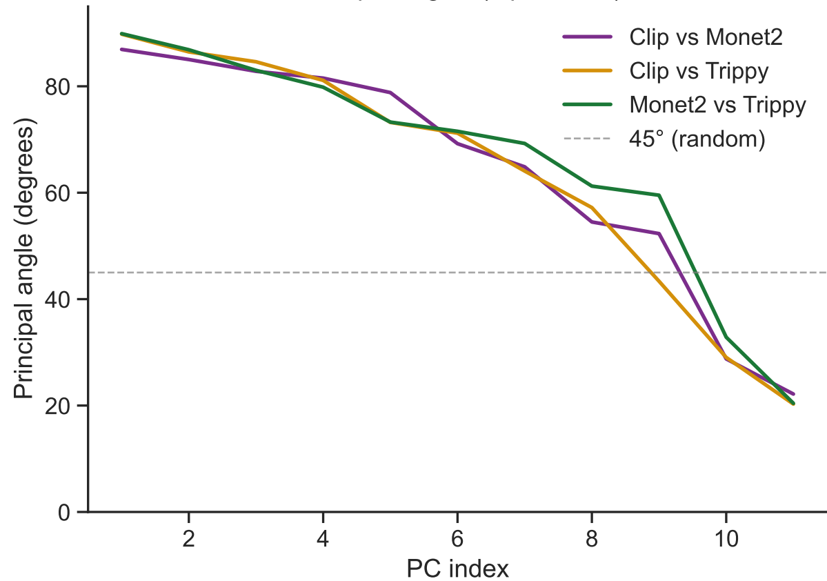
Principal angles (top-11 PCs)
