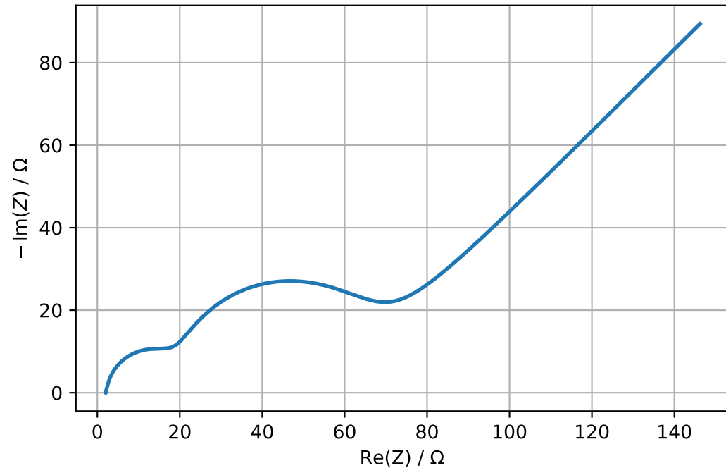
Nyquist plot
