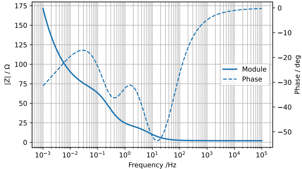
Bode plot
