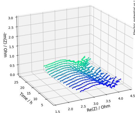
3D view of the oprando impedance
