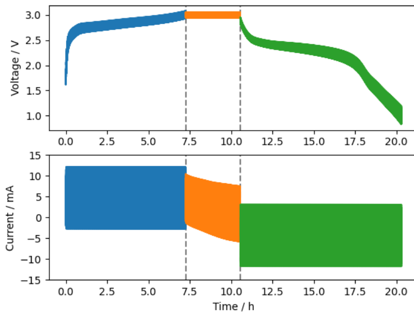
Figure 9.1: Voltage and current signals at 50 Sa/s after teh online computation step.
