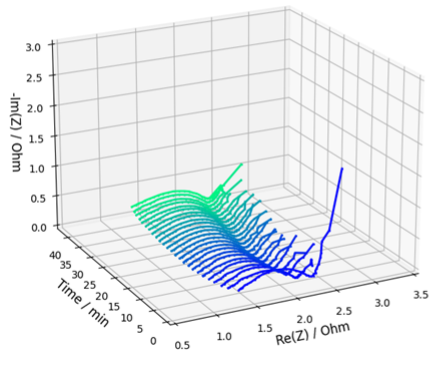
3D view of the oprando impedance
