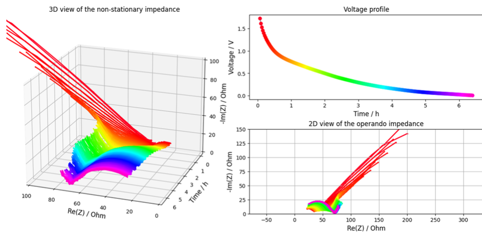
Figure 11.2: Cell 35 first discharge after formation.
