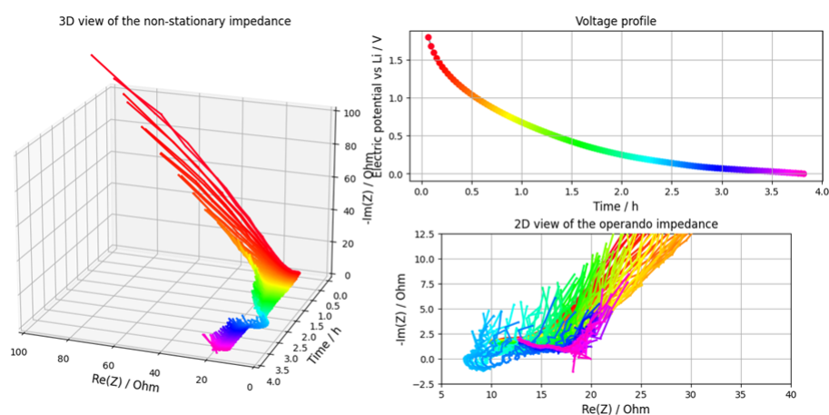
Figure 11.3: Cell 36 first discharge after formation.
