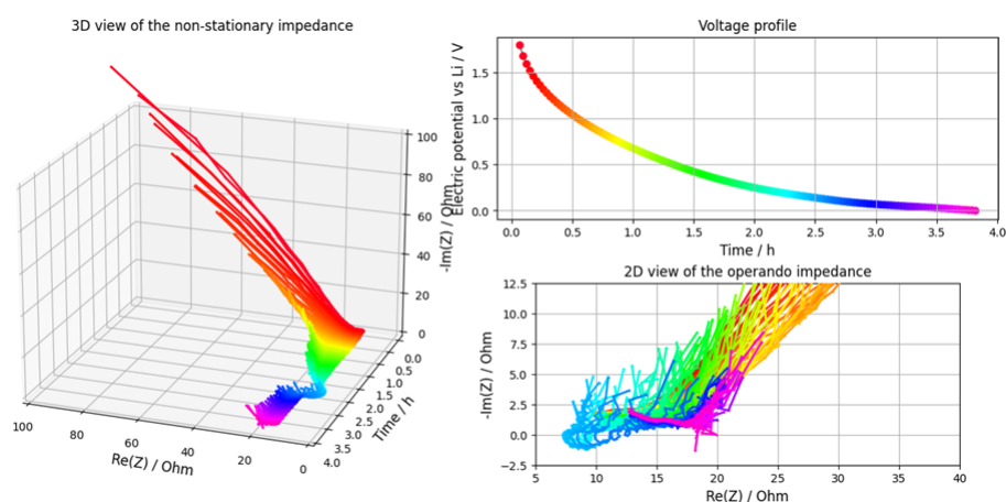
Figure 11.4: Cell 38 first discharge after formation.
