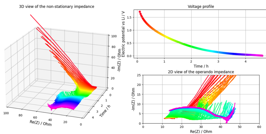
Figure 11.5: Cell 39 first discharge after formation.
