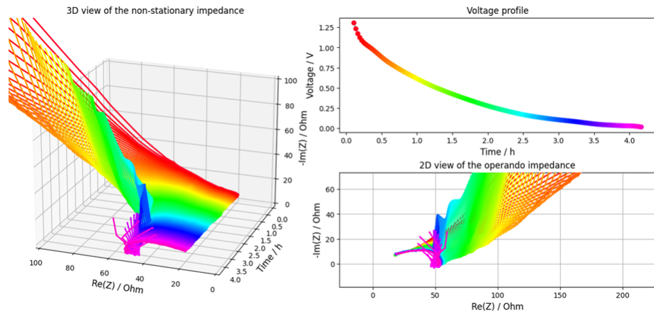
Figure 11.1: Cell 10 first discharge after formation.
