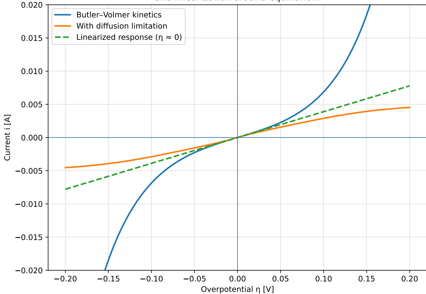
Butler-Volmer kinetics with diffusion limitation and linearization around equilibrium
