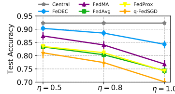
Figure 8: Test accuracy with different level of heterogeneity (ResNet18 on CIFAR-10).
