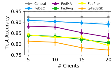
Figure 7: Test accuracy with different number of clients (ResNet18 on CIFAR-10).
