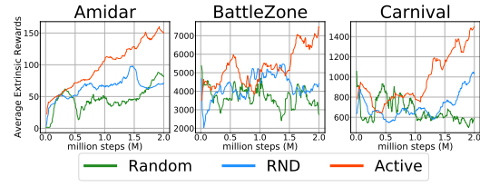
Figure 5: Comparisons on earned extrinsic rewards using random, RND, and our active exploration strategy respectively.
