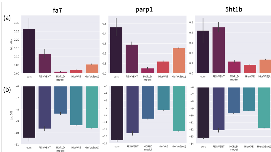
Figure 4: Hit ratio and top 5% score of our model FREED(PE), REINVENT, MORLD, HierVAE, and HierVAE(AL). Standard deviation is given as error bars. Higher hit ratios and greater negative value of the top 5% scores indicate better performance.
