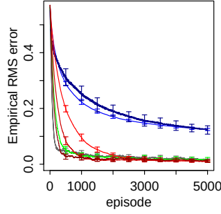
Figure 7: Performance of Gradient-DD in the random walk task when the initial values are set 0. The size of state space is 20, with tapering step size \alpha_n = 0.2(10^3 + 1)/(10^3 + n) . Results are averaged over 20 runs, with error bars denoting standard deviations across runs.
