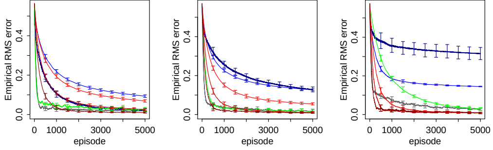
Figure 6: Performance of Gradient-DD in the random walk task under Case 3. Tapering step size \alpha_n = \alpha_0(10^3 + 1)/(10^3 + n) and \kappa is allowed to be dependent on n : \kappa_n = c\alpha_n . From left to right in each subfigure: the size of state space is 10 ( \alpha_0 = 0.1 ), 20 ( \alpha_0 = 0.2 ), 50 ( \alpha_0 = 0.5 ). Results are averaged over 20 runs, with error bars denoting standard deviations across runs.
