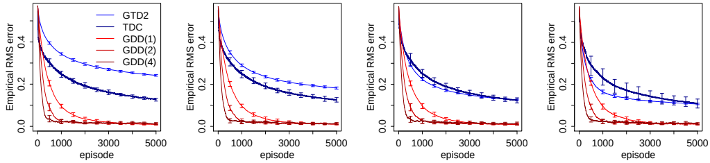
Figure 8: Performance under various \beta_n in the random walk task with 20 states. \alpha_n = \alpha_0(10^3 + 1)/(10^3 + n) with \alpha_0 = 0.2 . From left to right in each subfigure: the size of state space is \beta_n = \alpha_n/4 , \beta_n = \alpha_n/2 , \beta_n = \alpha_n , and \beta_n = 2\alpha_n . Results are averaged over 20 runs, with error bars denoting standard deviations across runs.
