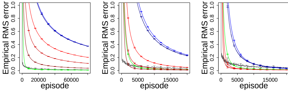
Figure 9: Performance of Gradient-DD in the Boyan Chain task with 20-features under Case 3. Tapering step size \alpha_n = \alpha_0(10^3+1)/(10^3+n) , where \alpha_0 = 0.3, 0.5, 0.8 , where \alpha_0 = 0.3, 0.5, 0.8 from left to right, and \kappa is allowed to be dependent on n : \kappa_n = c\alpha_n . Note that the case GDD(4), i.e. c = 4 , is not shown when it does not converge.
