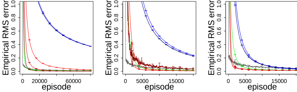
(b) Tapering step size \alpha_n = \alpha_0(10^3 + 1)/(10^3 + n) , where \alpha_0 = 0.3, 0.5, 0.8 from left to right.
