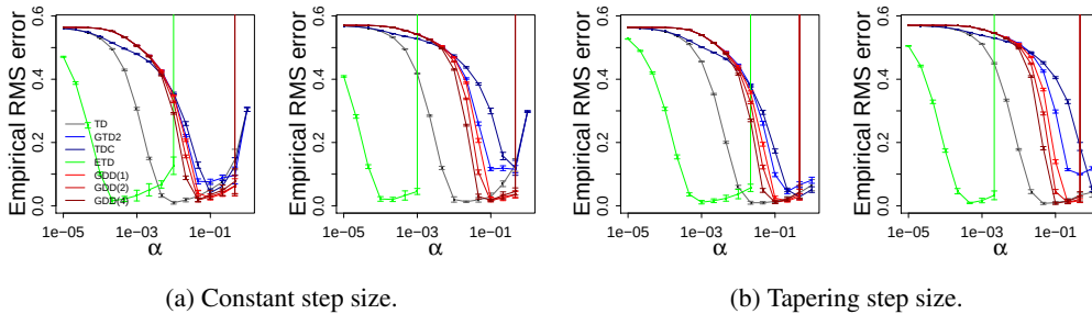
Figure 2: Performance in the random walk task depends on step size. (a), Constant step size \alpha_n = \alpha_0 . (b), Tapering step size \alpha_n = \alpha_0(10^3 + 1)/(10^3 + n) . In (a) and (b), state space size 10 (left) or 20 (right). GDD(c) denotes the Gradient-DD with c . The curves are averaged over 20 runs, with error bars denoting standard deviations across runs.
