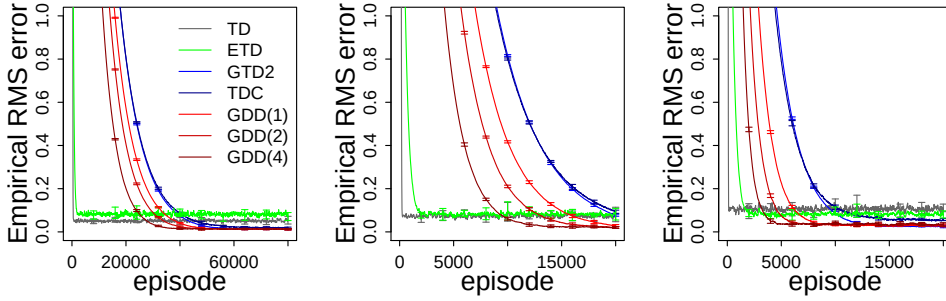
(a) Constant step size \alpha_n = \alpha_0 , where \alpha_0 = 0.05, 0.1, 0.2 from left to right.
