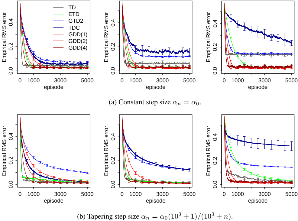
Figure 3: Performance of Gradient-DD in the random walk task. From left to right in each subfigure: the size of state space is 10 ( \alpha_0 = 0.1 ), 20 ( \alpha_0 = 0.2 ), 50 ( \alpha_0 = 0.5 ). The curves are averaged over 20 runs, with error bars denoting standard deviations across runs.
