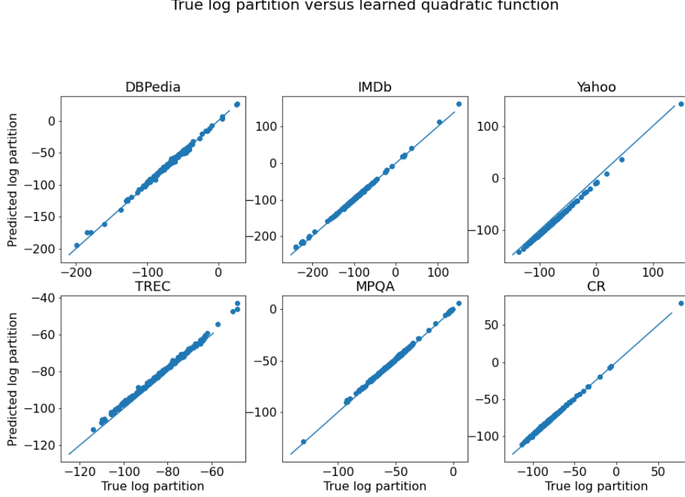
Figure 2: Fit of the learned quadratic function to the log partition function on various datasets for features computed by the full, pre-trained GPT-2. We also plot the y = x line for reference. These plots are meant to verify Assumption 4.1.
