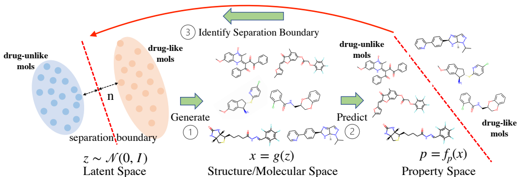
Figure 1: MolSpacE framework: (1) the tested molecule generative model generates novel molecules by sampling random vector from the latent space and then feeding it into the generator, (2) off-the-shelf property prediction function is used to predict molecular properties from the molecular space, (3) MolSpacE identifies latent directions which govern molecular properties via the property separation hyperplane.
