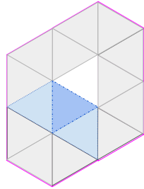
Figure 5: The two blue dashed cycles are homologically equivalent, the pink isn't.
