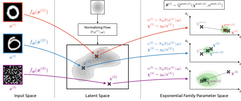
Figure 2: Overview of Natural Posterior Network. Inputs x^{(i)} are first mapped to a low-dimensional latent representation z^{(i)} by the encoder f_\phi . From z^{(i)} , the decoder g_\psi derives the parameter update \chi^{(i)} while a normalizing flow \mathbb{P}_\omega yields the evidence update n^{(i)} . Posterior parameters are obtained from a weighted combination of prior and update parameters according to n^{\text{post},(i)} .
