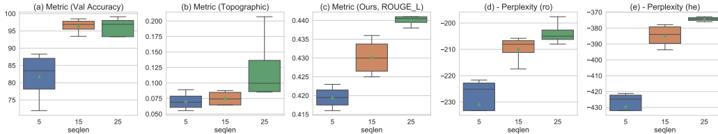
Figure 8: How metrics and downstream performances change with respect to sequence length (5, 15, 25). Vocabulary size is 4035 and training step is 1000.
