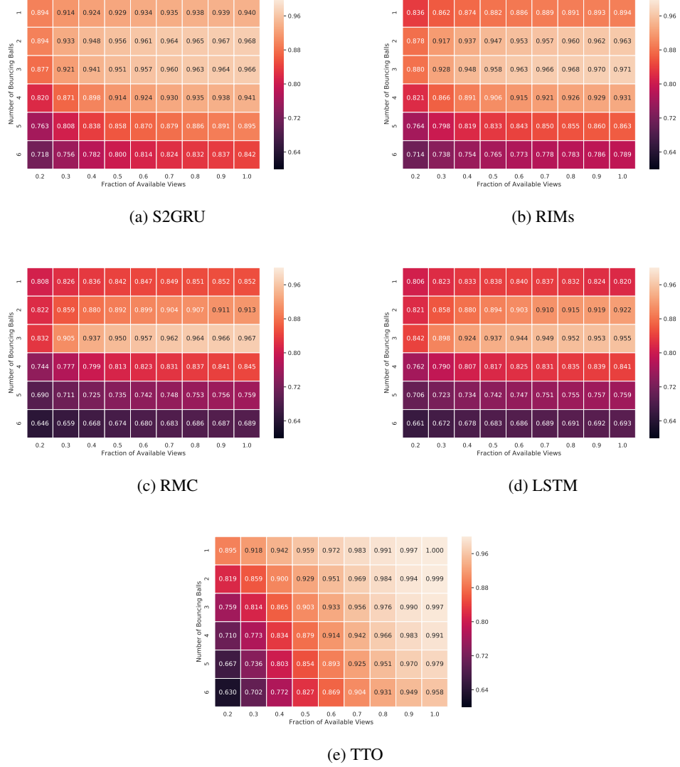
Figure 21: F1-Score (harmonic mean of precision and recall) achieved by all evaluated models for one-step forward prediction task with various number of balls and fractions of available views. All models were trained on video sequences with 3 balls and a constant number of crops / views (10 views, corresponding to the right-most columns labelled 1.0). The color map is consistent across all plots.
