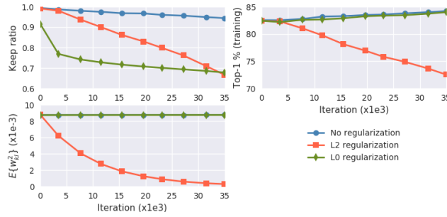
Figure 2: Ablation study with various regularization methods for ResNet20 on Cifar100. Keep-ratio (upper-left), training Top-1 (upper-right) and mean-squared-weights for layer3.2.conv2 (lower-left).
