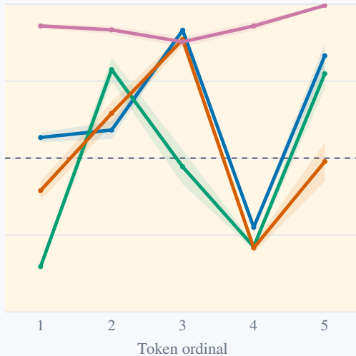
Boundary
