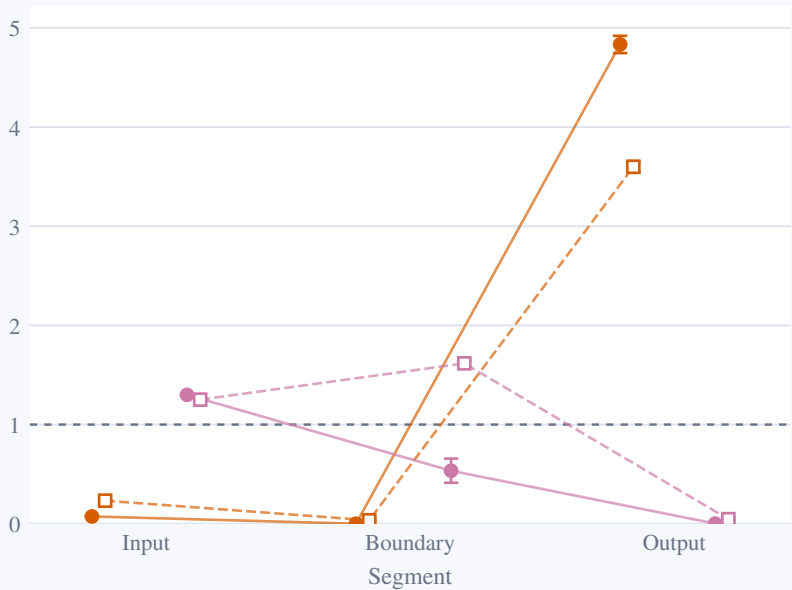
High-rank enrichment
