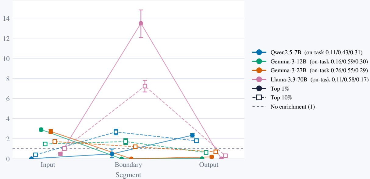
High-rank enrichment
