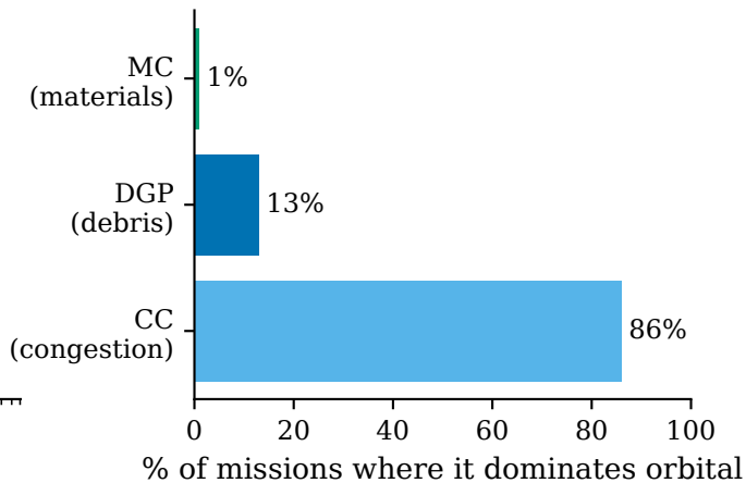
(b) Dominant orbital driver (reference normalisation)
