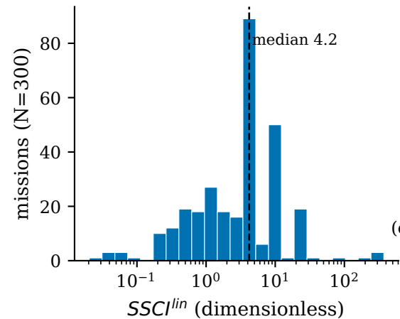
(a) SSCI distribution over the catalogue
