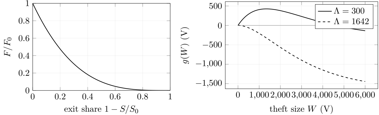
Figure 2: Left: fund retention under a discounted run, F/F_0 = (S/S_0)^{1/\rho^*} with \rho^* = 0.3 (Theorem 3) — positive at every exit share. Right: the fraud-profit bound g(W) at c = 1 (Theorem 5); the default stake \Lambda = 300 V leaves a profitable region peaking at \approx +425 V, while the threshold stake \Lambda = 1642 V makes every theft size loss-making.
