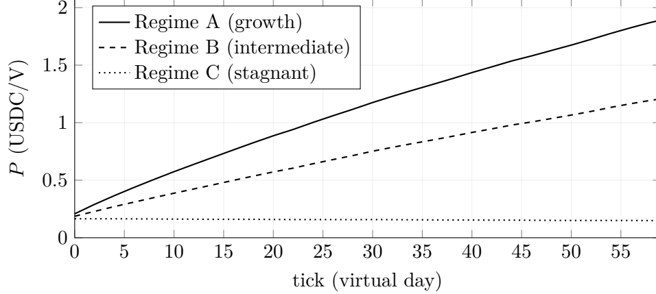
Figure 1: Simulator price trajectories for the three regime configurations (seed 23, 60 ticks; data from the released regime_analysis protocol). The growth and stagnant regimes behave as predicted; the intermediate configuration rises rather than holding flat, reflecting approximate calibration of inflows to emission.
