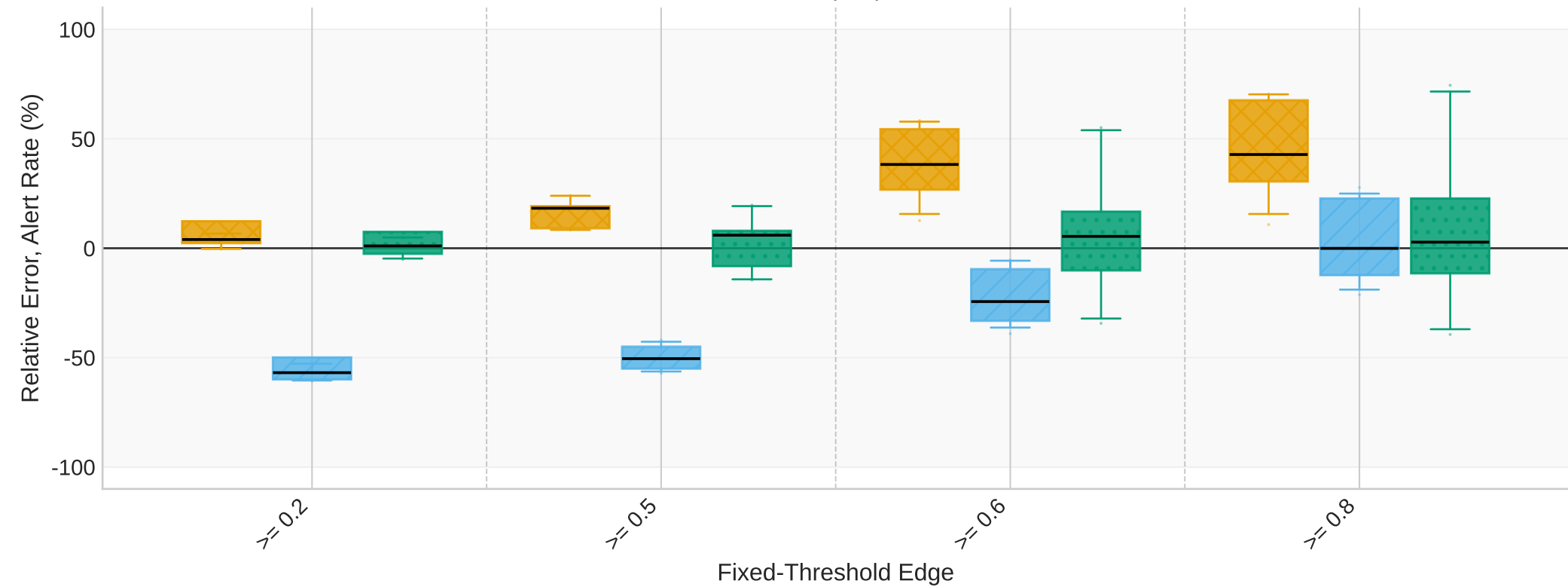
Alert-rate relative error, per predictor -- Variant II
