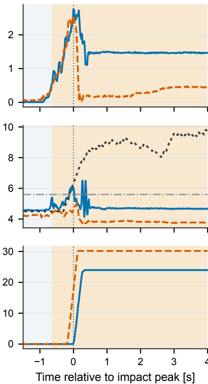
(b) Medium F_{E,pk} S/D: 2.58/2.76 N
