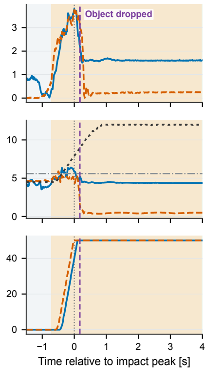
(c) High F_{E,pk} S/D: 3.75/3.80 N
