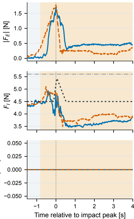
(a) Low F_{E,pk} S/D: 1.77/1.71 N
