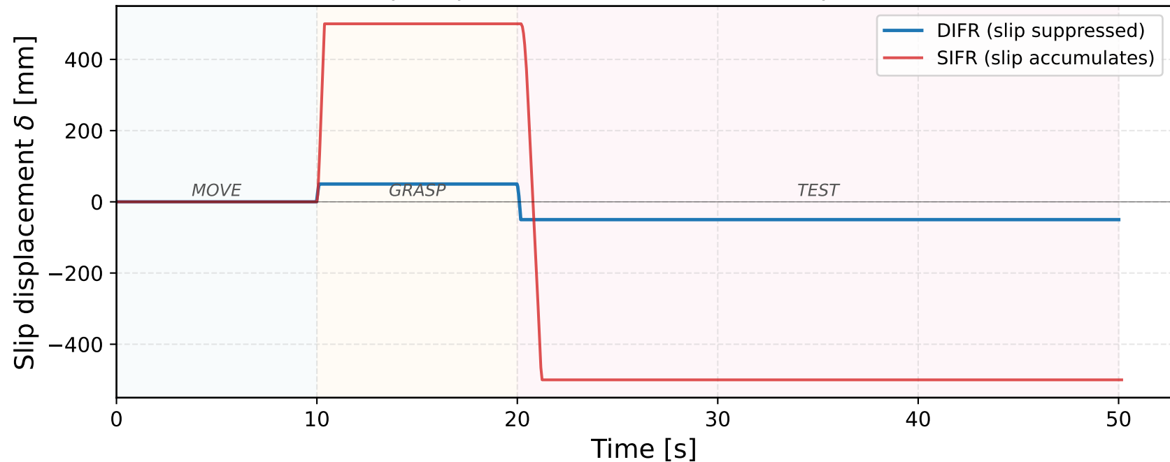
Slip Displacement: DIFR vs SIFR (Eq. 39-40)
