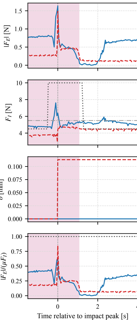
(a) Low F_{E, pk} S/D: 1.49/1.63 N
