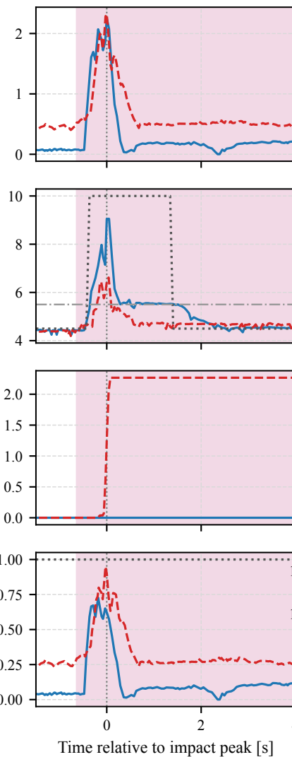
(b) Medium F_{E, pk} S/D: 2.32/2.26 N
