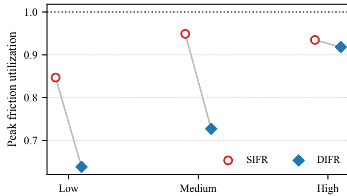
(c) Friction-cone margin
