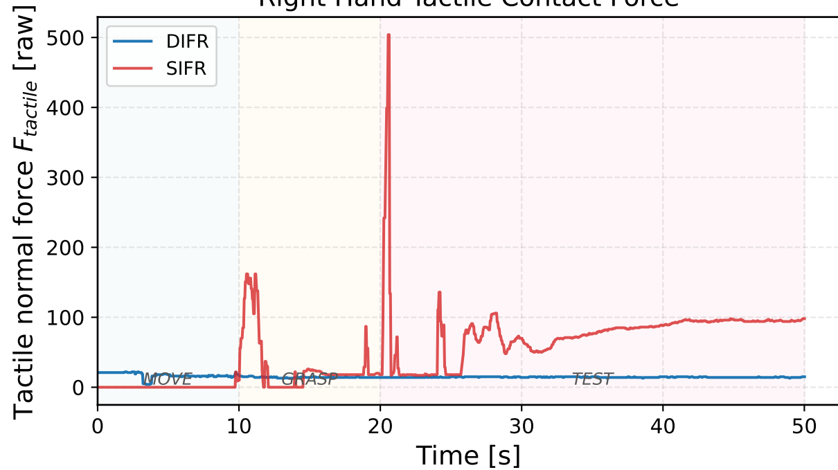
Right Hand Tactile Contact Force
