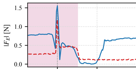
(a) Low - unmatched F_{E,pk} S/D: 1.18/1.55 N
