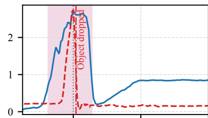
(c) High F_{E,pk} S/D: 2.73/2.74 N
