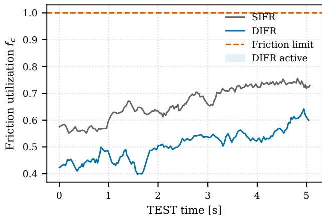
(c) Friction-cone utilization
