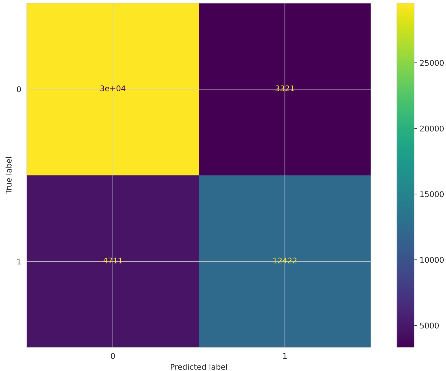
Confusion Matrix - DNN
