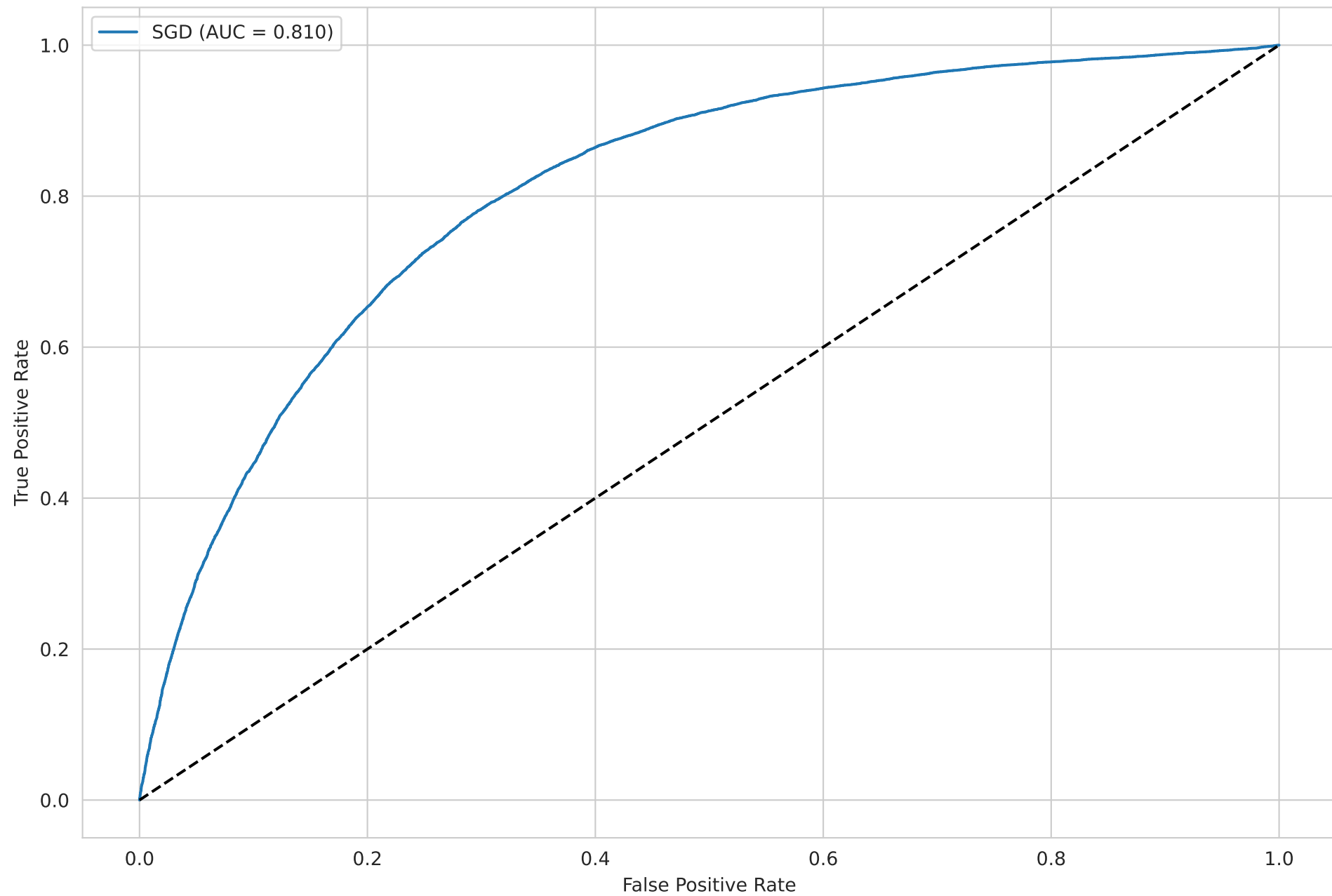
ROC Curve - SGD
