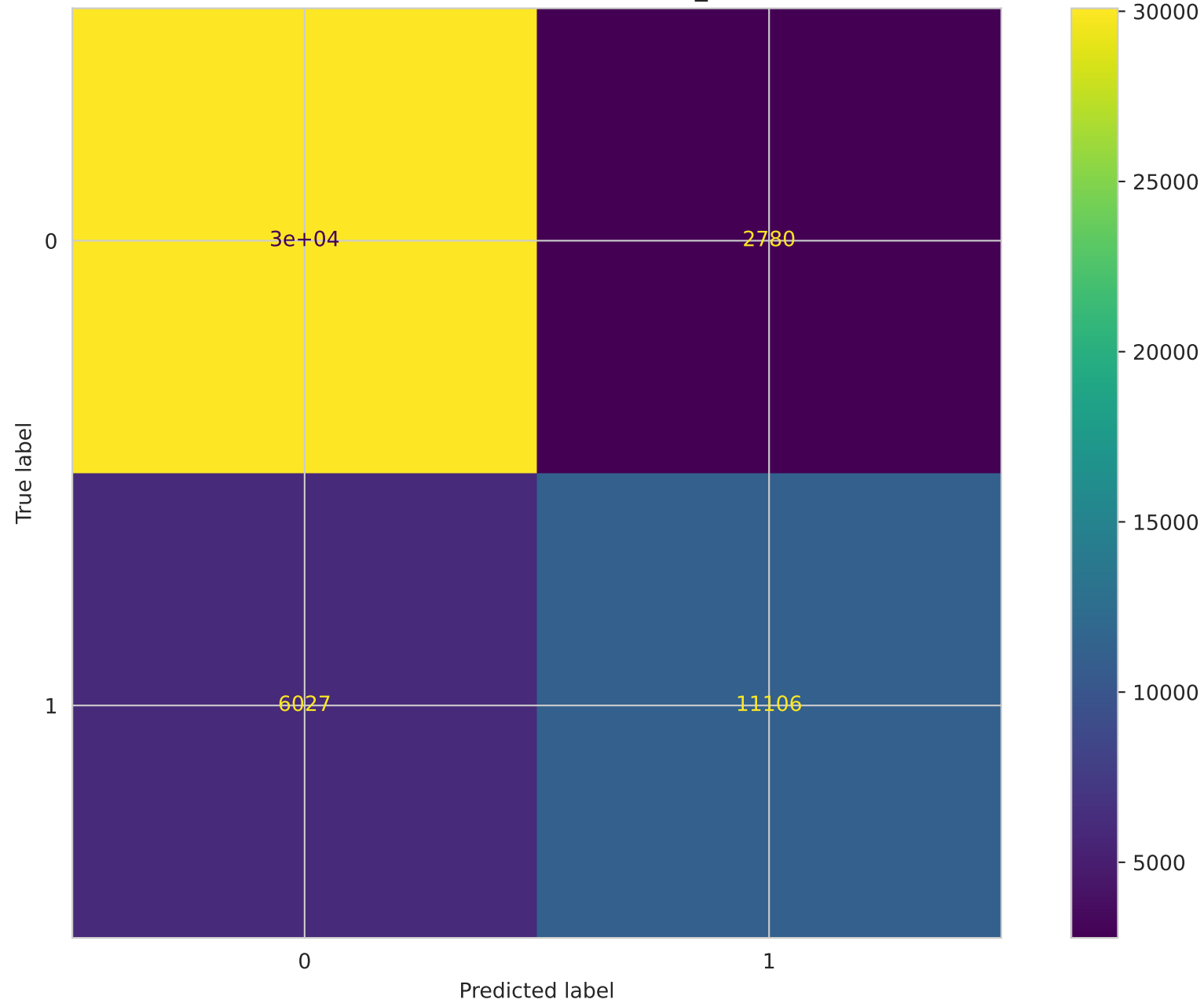
Confusion Matrix - XGBoost_2
