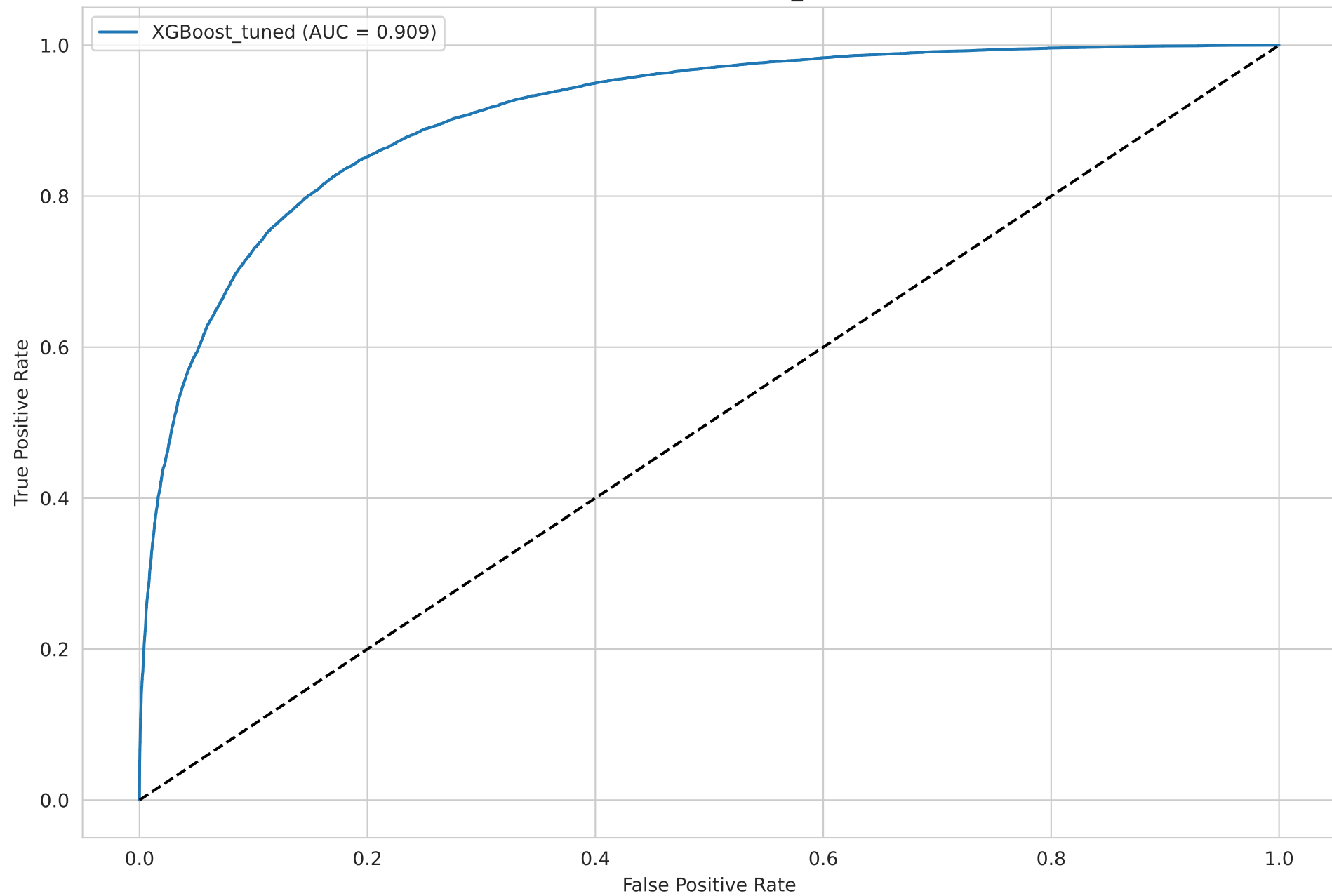
ROC Curve - XGBoost_tuned
