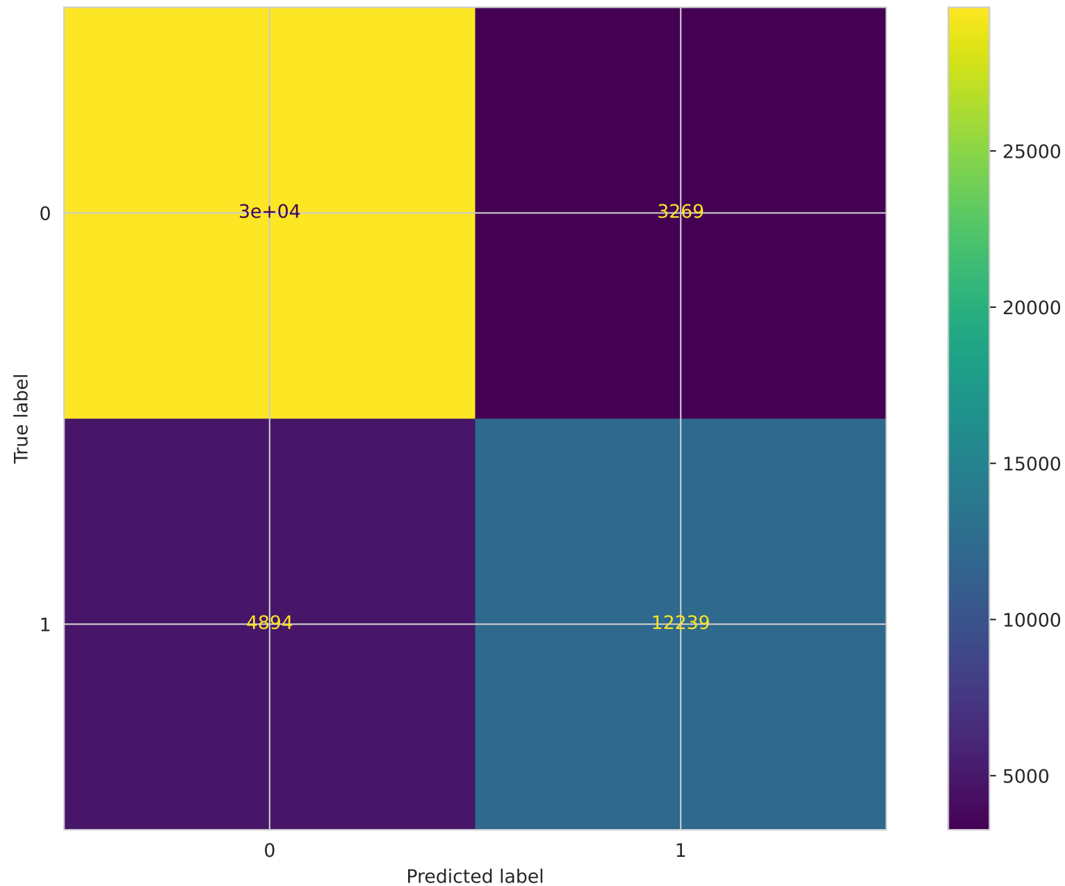
Confusion Matrix - XGBoost
