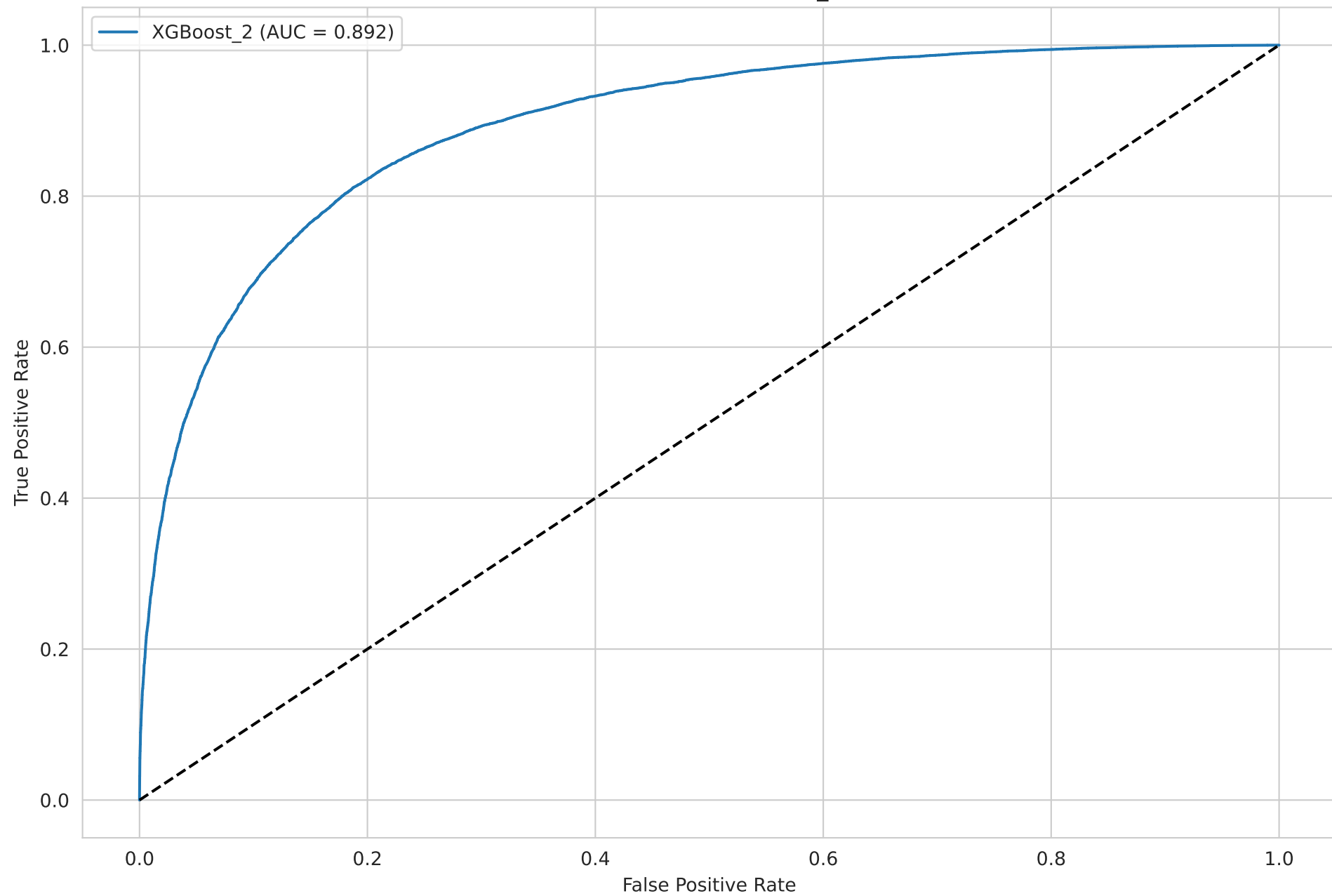
ROC Curve - XGBoost_2
