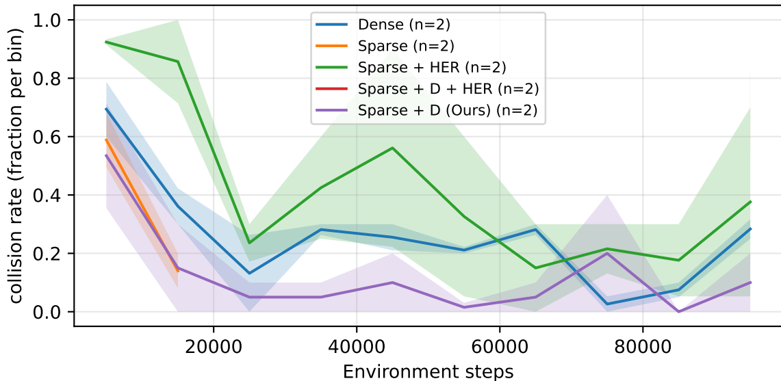
Lane Following — collision rate vs Env Steps
