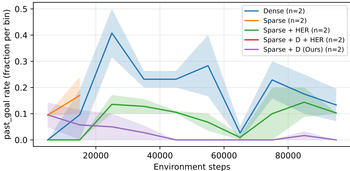
Lane Following — past_goal rate vs Env Steps
