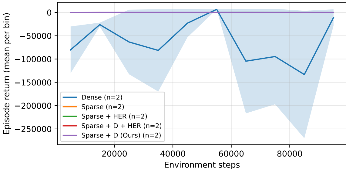
Lane Following — Return vs Env Steps
